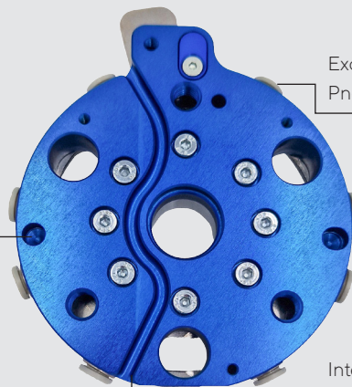
H7 centering holes for exact positioning on the robot
